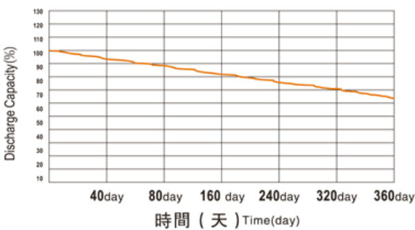
在常溫下LYP類電池的存儲特性曲線 Storage characteristic curve of LYP type battery under normal temperature
